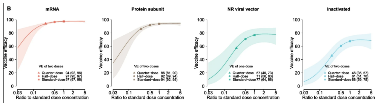
Figure. An illustration of an uncertain, model-derived relationship for COVID-19 vaccines. You can ignore the implications for COVID, the general point is that for a given vaccine many lower doses can lie either on “top” of the S or close to it. (For more on COVID specifically, also see this study.) Also note that this figure focuses on the magnitude of immediate response, but durability of protection is also an important consideration: again, this is intended as a generic illustration of saturating curves.
